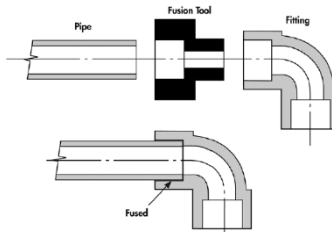
FIG. 1 Socket Fusion
